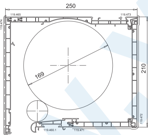
VEKAVARIANT 210
