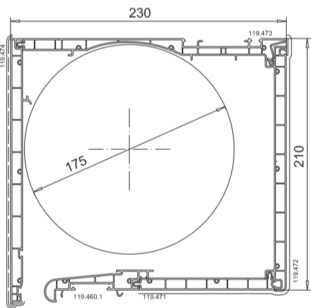
VEKAVARIANT 210
