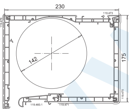
VEKAVARIANT 175
