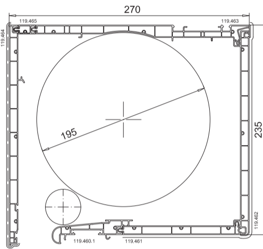
VEKAVARIANT 235
