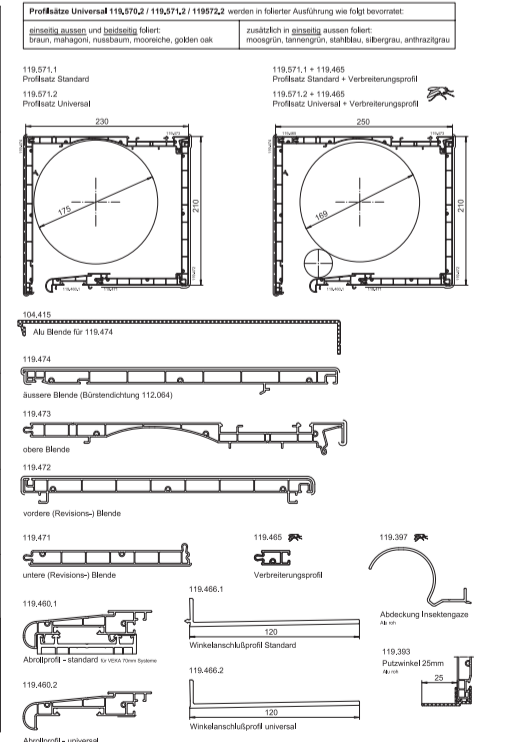
VEKAVARIANT 210
