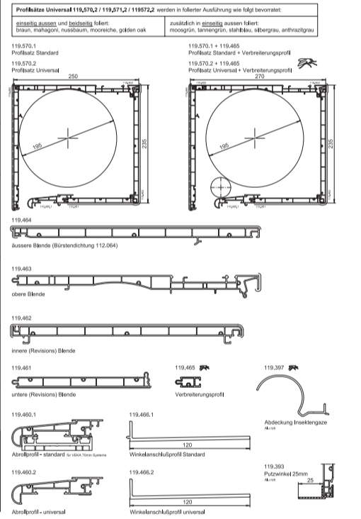
VEKAVARIANT 210
