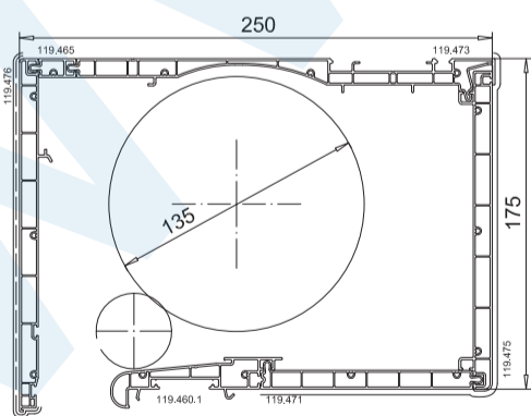
VEKAVARIANT 175
