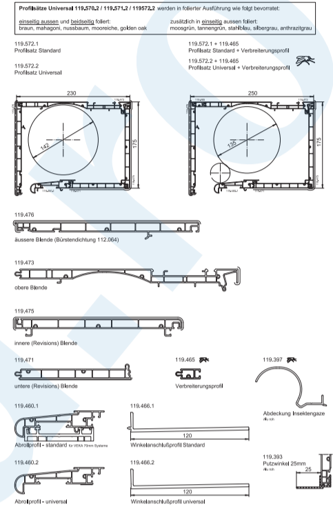
VEKAVARIANT 175
