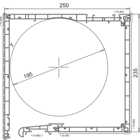
VEKAVARIANT 235
